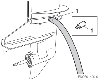
1. Flushing attachment
