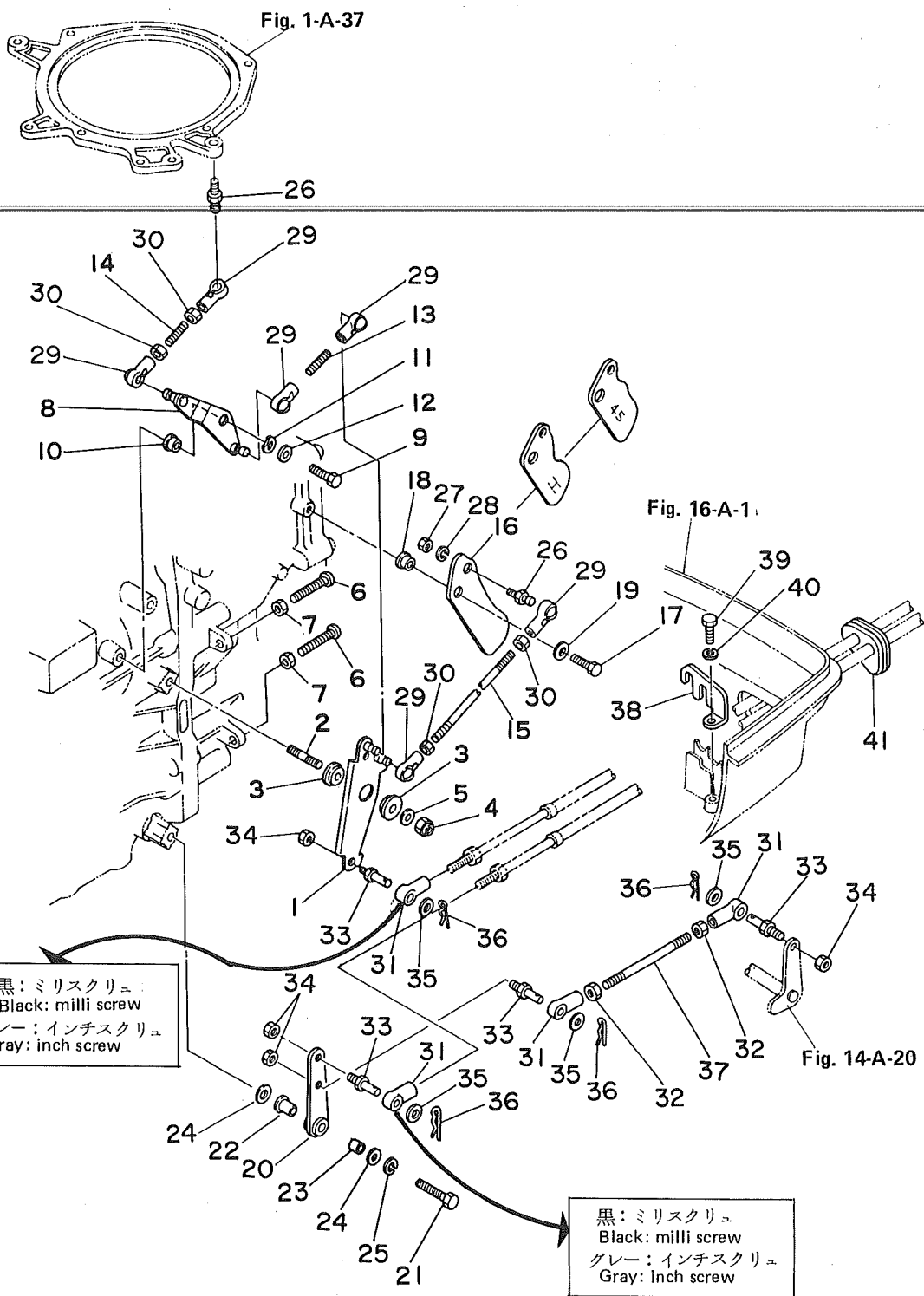
Fig. 7-A THROTTLE MECHANISM (I) "P" TYPE
