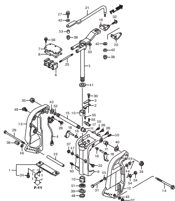
F-10 STERN BRACKET/SWIVEL CASE
