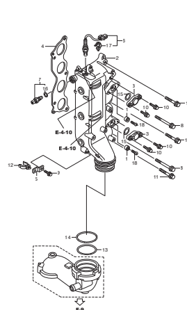
E-4 EXHAUST PIPE
